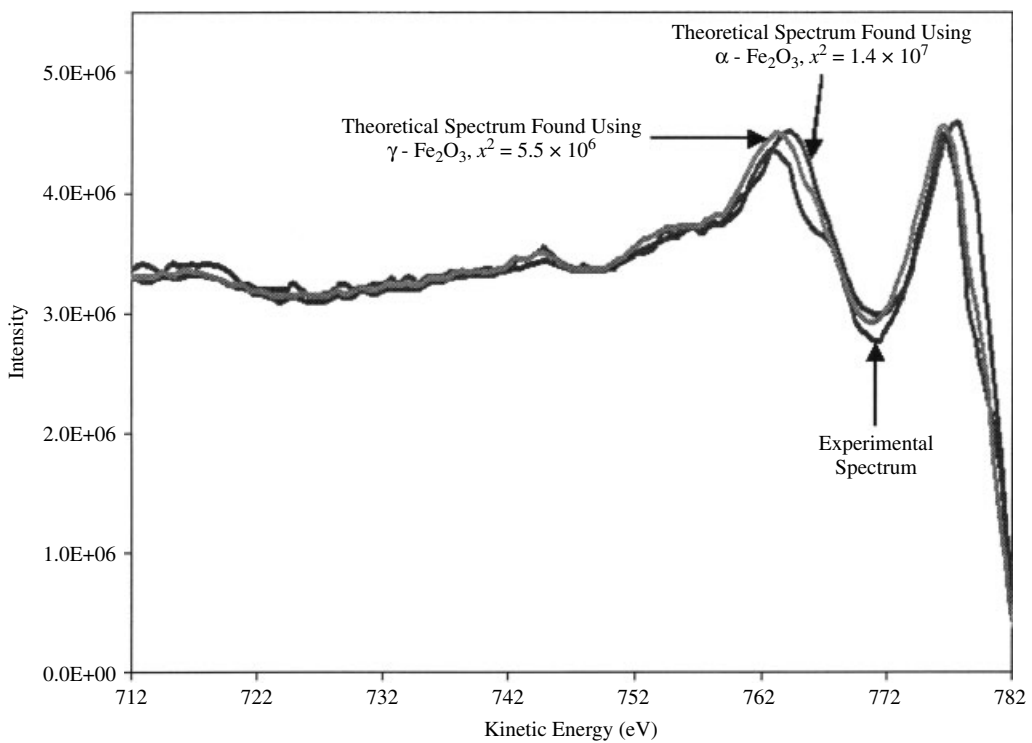
Figure 4. Graph of the experimental and theoretically modelled Fe 2p results discussed above for the Fe surface exposed to dry air for 2 h, along with their chi-squared values, indicating the modelled spectra's goodness of fit. Both the \gamma - and \alpha -Fe 2 O 3 spectra were shifted upwards by 2 eV to achieve the best fit.
