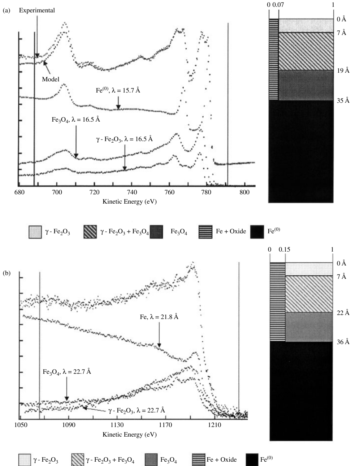
Figure 6. (a) The Fe 2p QUASES™ Generate results of 120 s air-exposed Fe surface analysed using an Al K \alpha x-ray source. The model spectrum used for \gamma\text{-Fe}_2\text{O}_3 was shifted upwards by 2.5 eV to achieve the best fit. (b) The Fe 2s QUASES™ Generate results of 120 s air-exposed Fe surface analysed using a Zr L x-ray source. All three model spectra used were shifted to a lower kinetic energy by 0.5 eV to achieve the best fit. The model and experimental spectra overlap each other to a point where they are indistinguishable.
